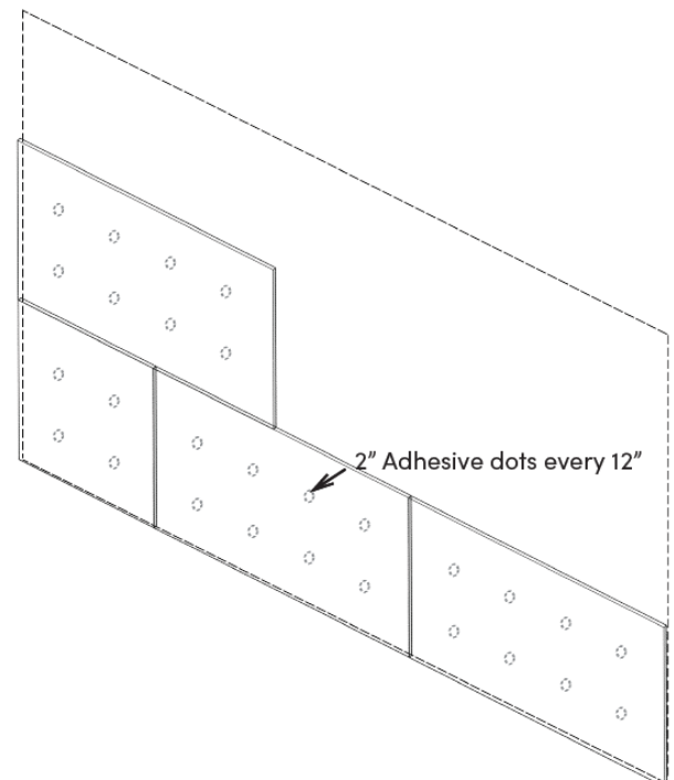
Butt Joint
