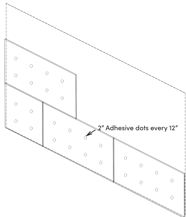
Butt Joint
